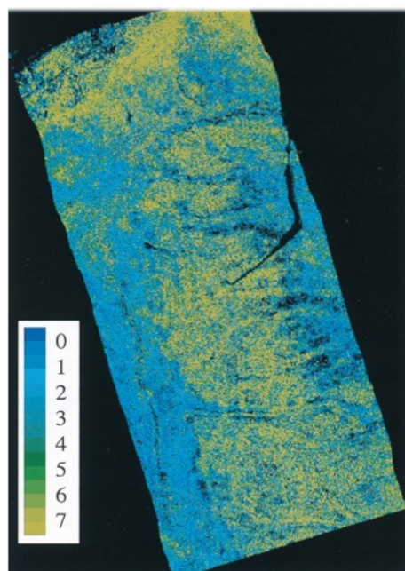
Plate 1. CASI-LAI image of a black spruce stand, BOREAS tower site SOBS, located near Candle Lake, Saskatchewan, Canada. The image is obtained after several steps of image processing (see text) based on the SR-LAI relationship derived using transect measurements at the same site.
